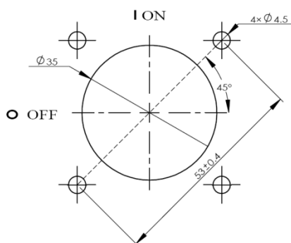
柜门安装孔尺寸 Panel drilling
